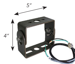
LF3-YOK Adjustable U-shaped yoke mount with 20" wire & strain relief connector (LF3-80, 100, 150, 220 & 300)
