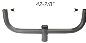
PT2-180 Double in-line at 180°, 1' (H), 3' between centers, slips on 2-3/8" pole
