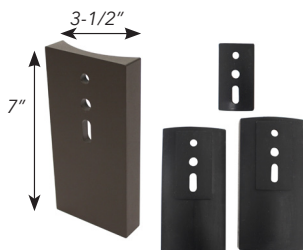
PSR4 Adapter kit for 3", 4" and 5" round poles. Separate gasket provided for each size pole.
