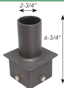
PSS3SVTZ (3") PSS4SVTZ (4") PSS5SVTZ (5") 3" or 4" or 5" square pole vertical tenon, bronze. Goes on 3" or 4" or 5" pole to accept 2" slip fitter.
