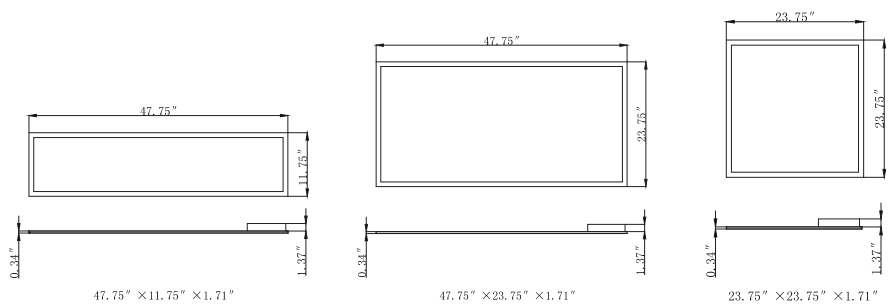
Emergency System Pre-installed (In 1X4 Installed but not attached to fixture)
