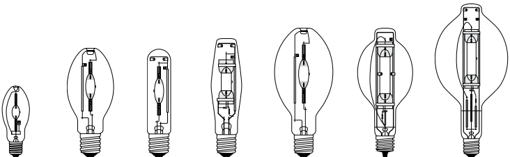
ED17/E26 ED28/E39 T15/E39 ET18/E39 ED37/E39 BT37/EX39 BT56/E39
